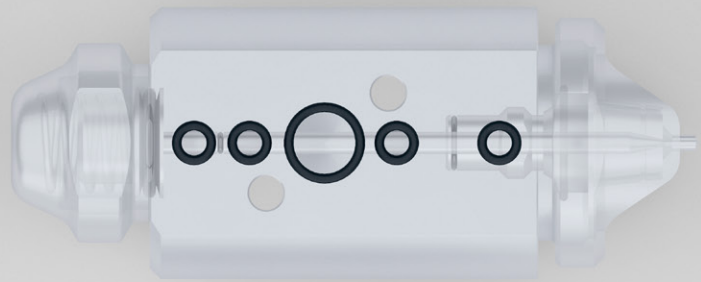
PCA nozzles with standard O-rings
